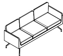
Three Seater L 1800 x D 665 x H 780
