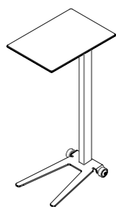
L 450 x D 500 x H 1000 mm
