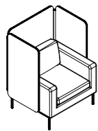
Single Seater L 900 x D 815 x H 1200 mm
