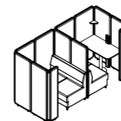
2+2 Seater L 2980 x W 1320 x H 1650 mm
