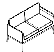
Two & Half Seater L 1500 x D 665 x H 780
