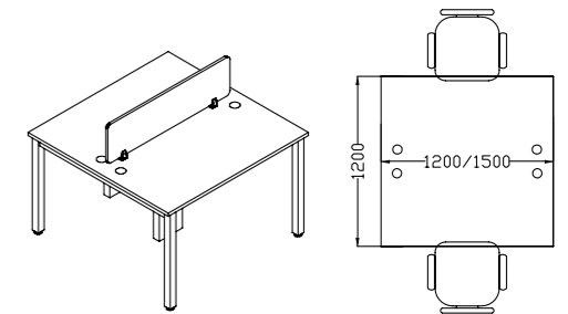
2 Seater 1200x1200 / 1500x1200
