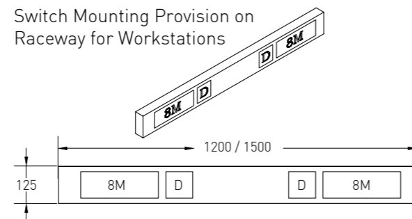
Cutout Details (Standard Anchor Roma)
