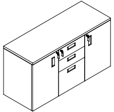
Side Unit 1200Wx450Dx640HT
