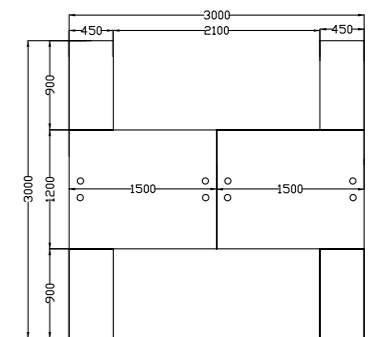
4 Seater Main: 3000x3000 | Return: 900x450
