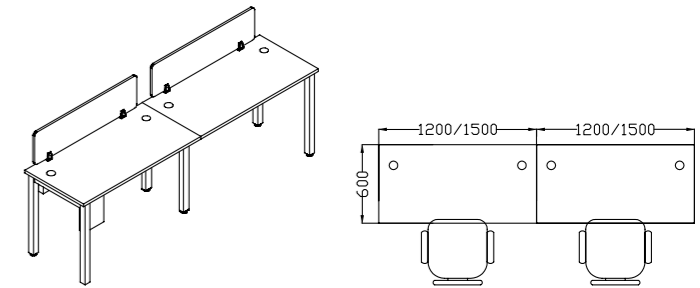
2 Seater 2400x600 / 3000x600
