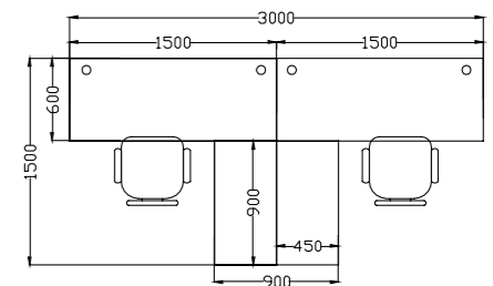
2 Seater (b) Main: 3000x1500 | Return: 900x450
