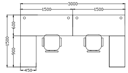
2 Seater (a) Main: 3000x1500 | Return: 900x450
