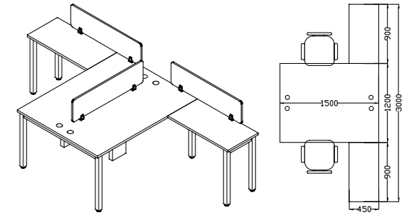
2 Seater Main: 1500x600 | Return: 900x450
