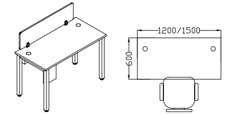
1 Seater 1200x600 / 1500x600
